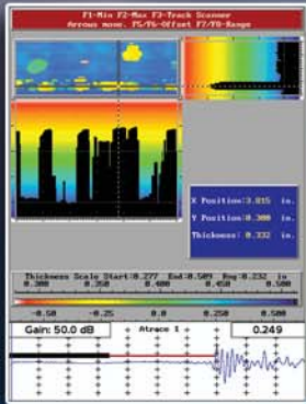
A&B-Scan
